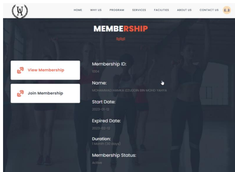
Figure 24: Membership Page
