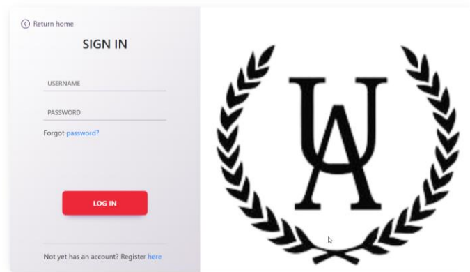
Figure 18: Login Page
